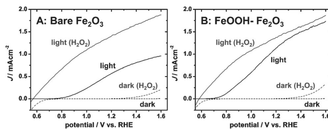
Figure 4. J – V curves for the A) bare Fe 2 O 3 and B) FeOOH/Fe 2 O 3 photoanodes. For photo-oxidation of the hole scavenger, a NaOH (1 M) electrolyte containing H 2 O 2 (0.5 M) was used under 1 sun irradiation.
